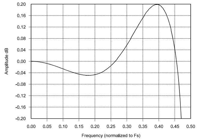
Figure 22. Passband Ripple
